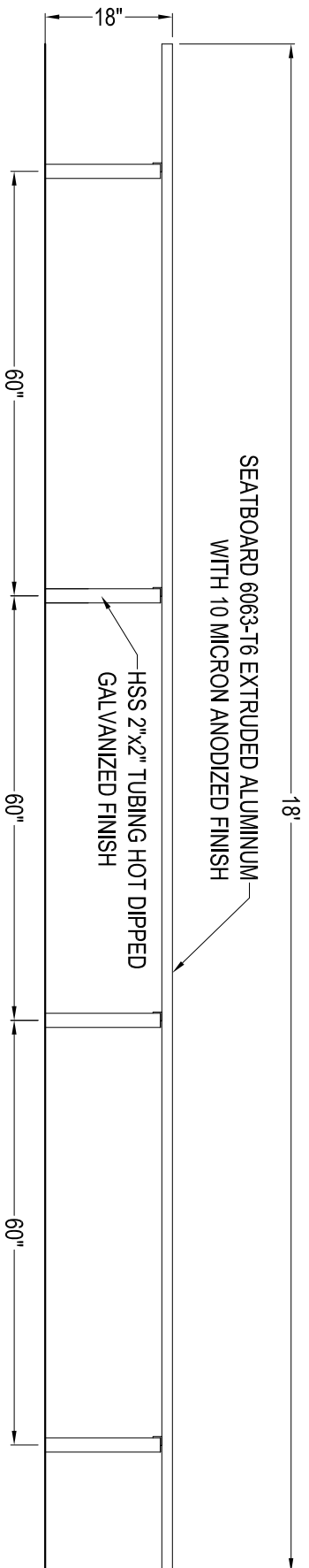
SIDE ELEVATION BL-SM-18 SCALE: 1/2" = 1'
