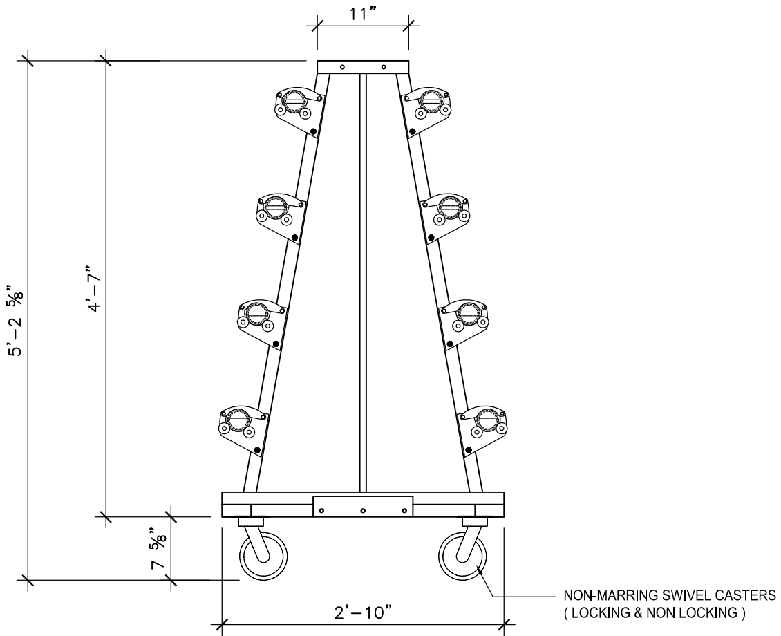
END ELEVATION : FLOOR COVER RACK SCALE: 3/4" = 1' (UNLOADED)
