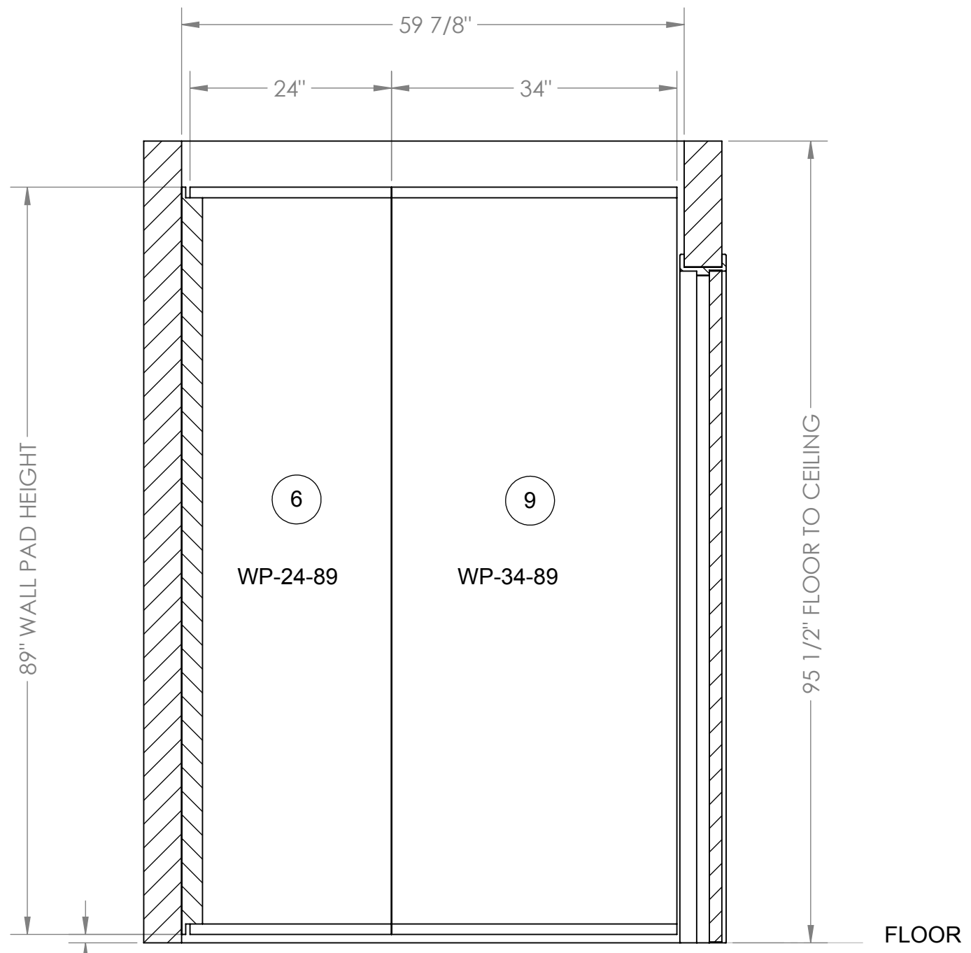
ELEVATION RIGHT WALL SCALE 1 : 16
