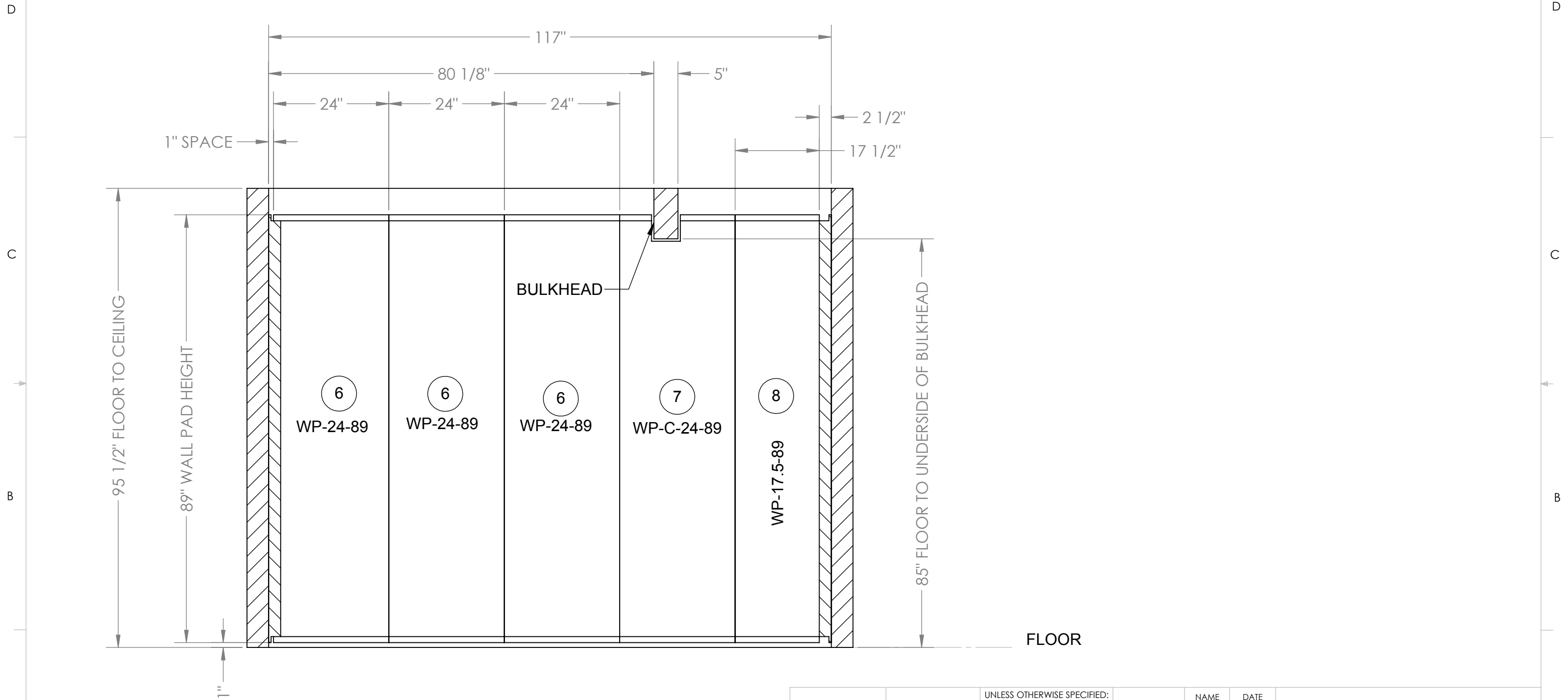
ELEVATION REAR WALL SCALE 1 : 20
