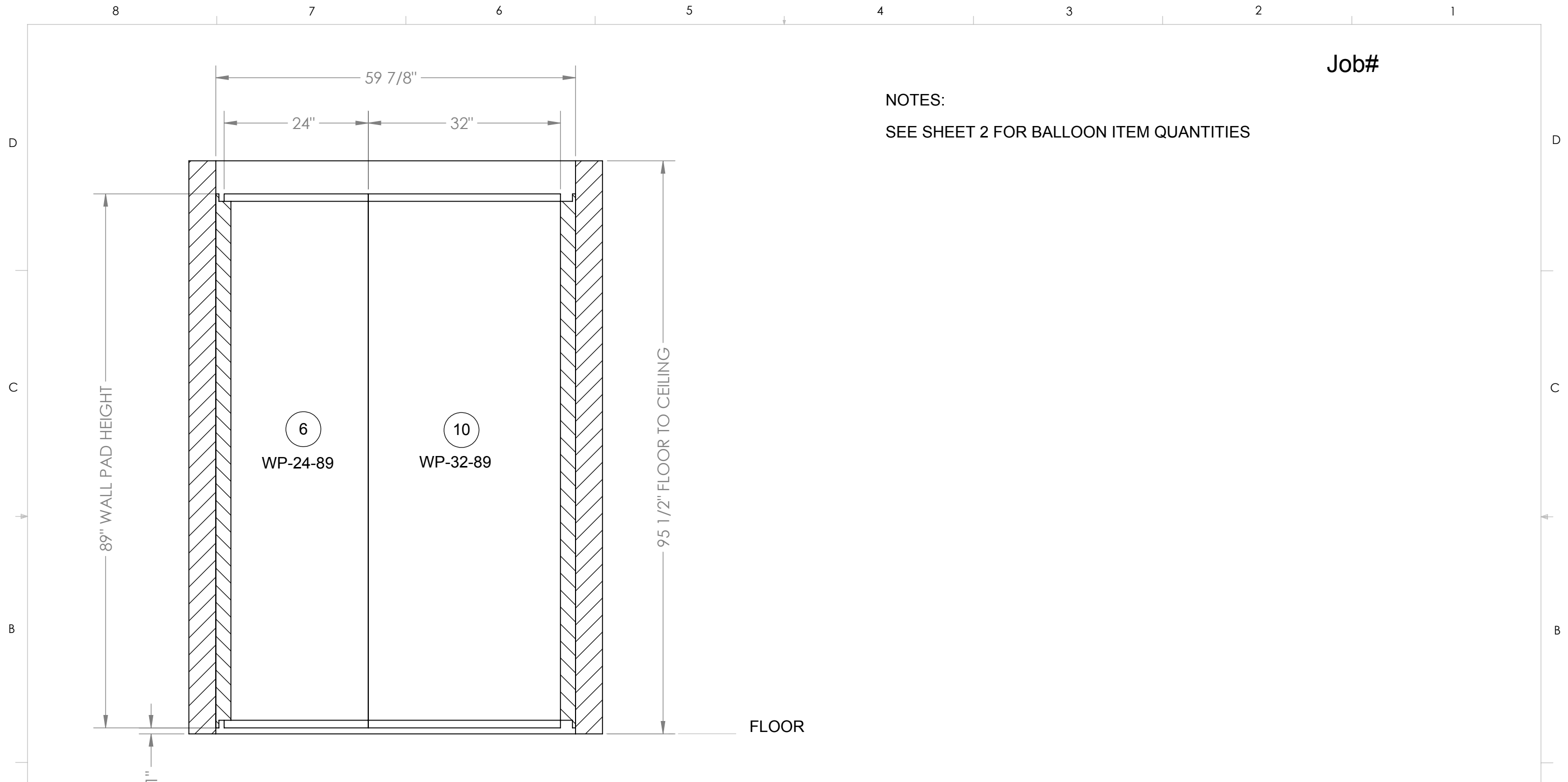
ELEVATION LEFT WALL SCALE 1 : 16
