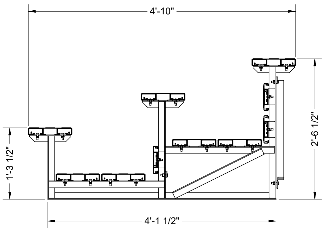
SECTION THROUGH BLEACHER SEATING
