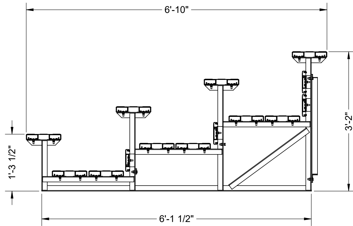
SECTION THROUGH BLEACHER SEATING
