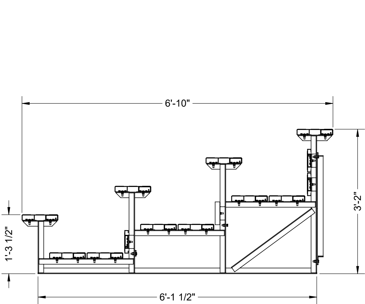
SECTION THROUGH BLEACHER SEATING
