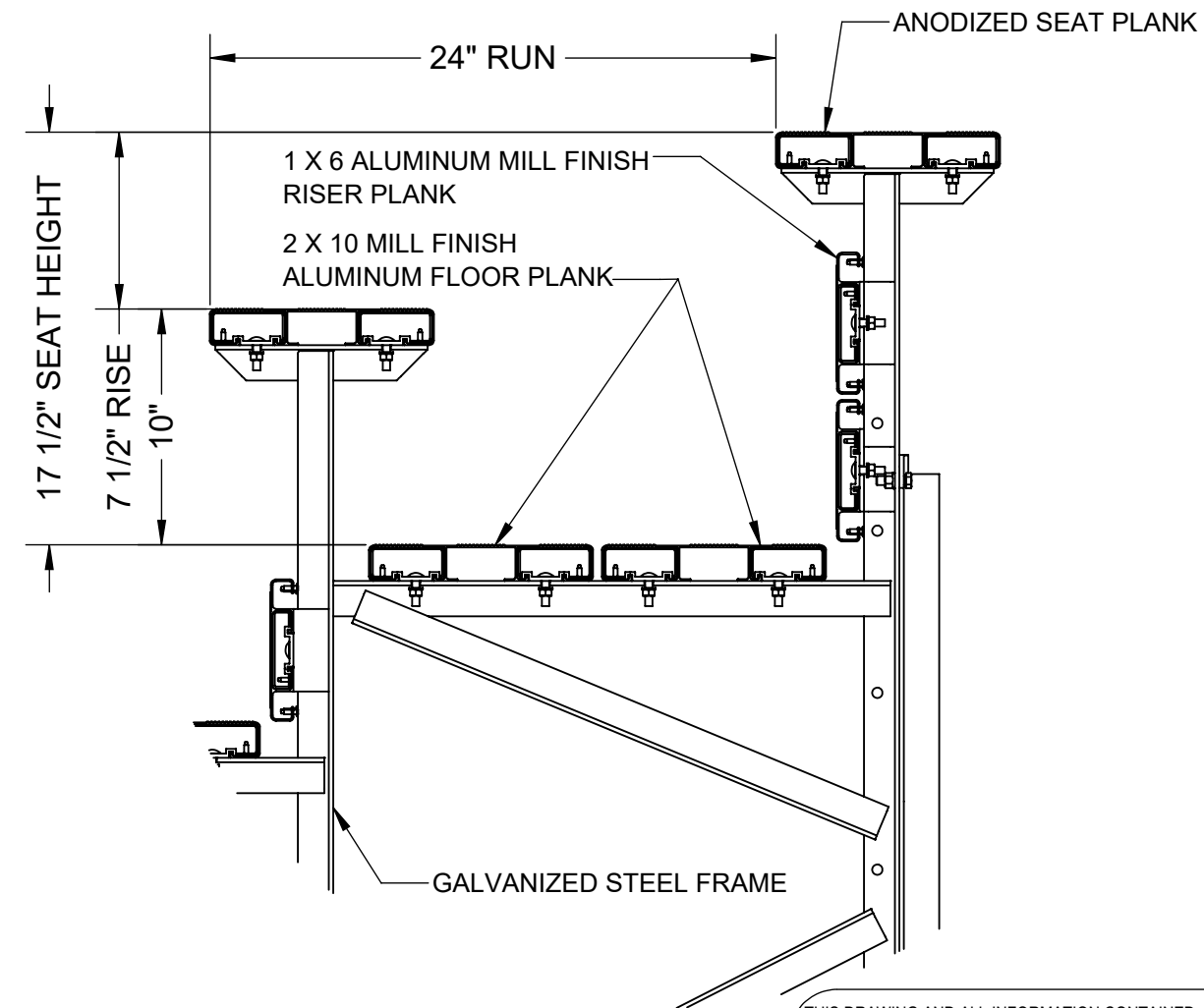
TYPICAL SEAT AND FLOOR BOARD DETAIL NOT TO SCALE
