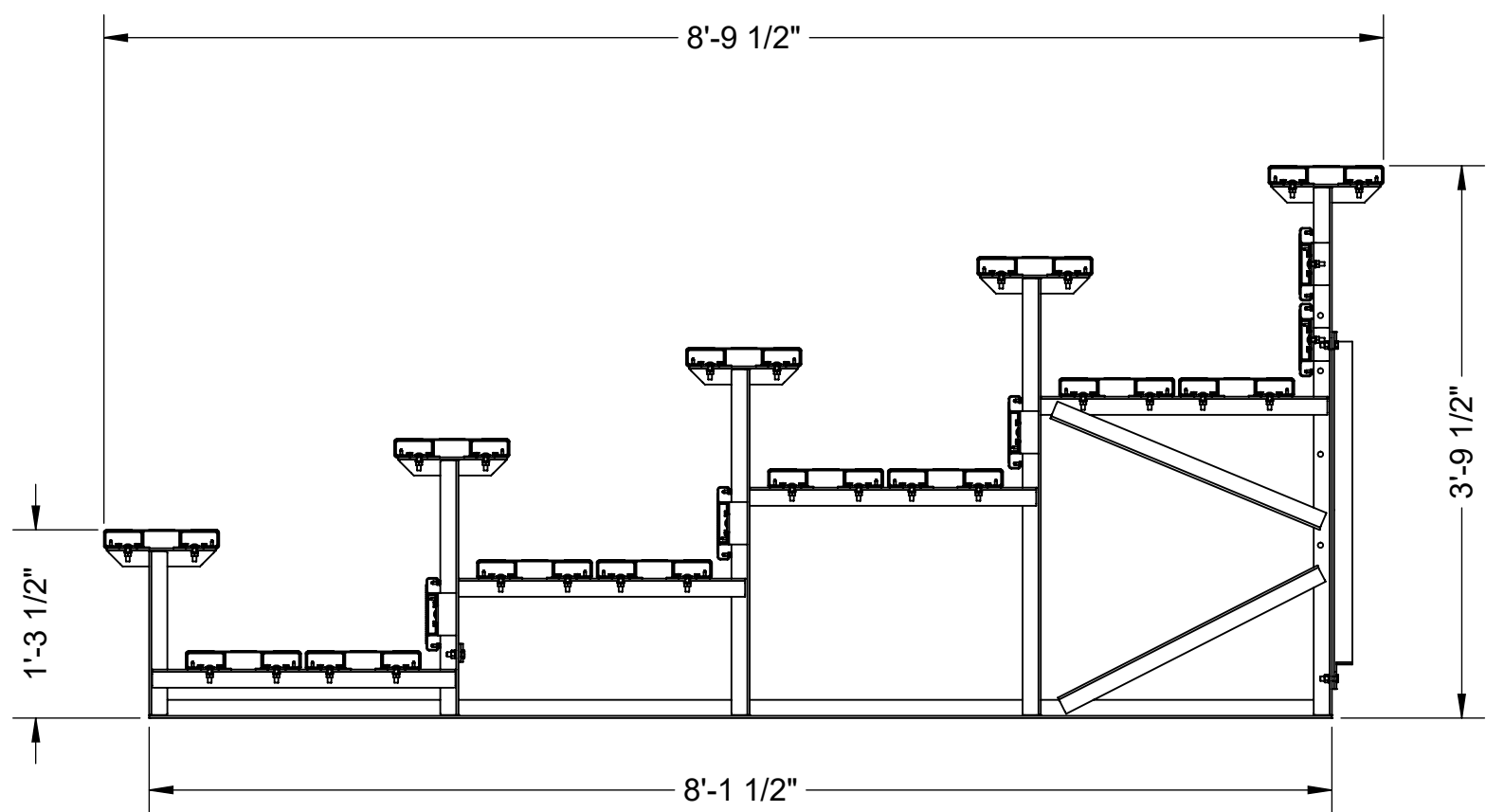
SECTION THROUGH BLEACHER SEATING
