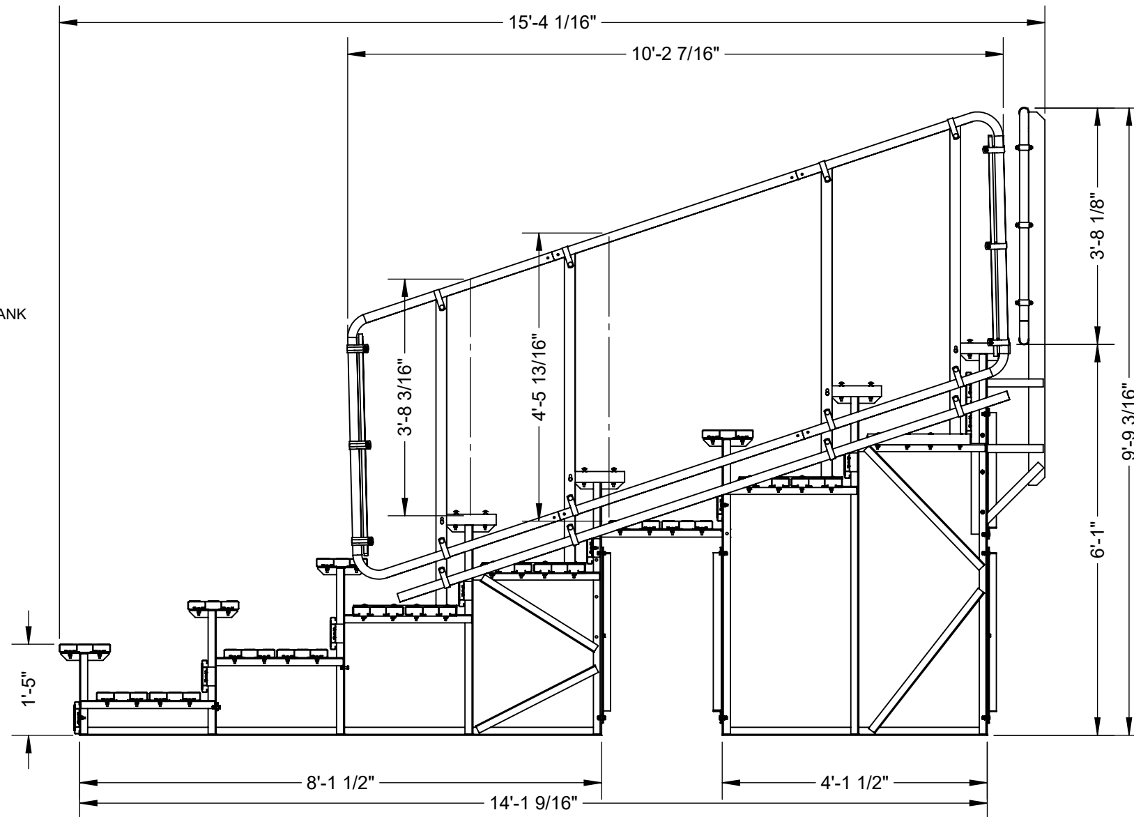
SECTION THROUGH BLEACHER SEATING
