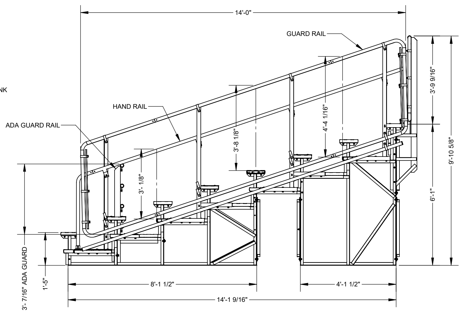
SECTION THROUGH BLEACHER SEATING NOTE: CHAIN LINK REMOVED FOR CLARITY
