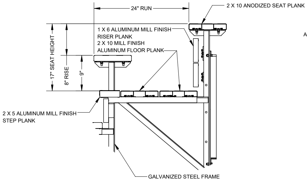
TYPICAL SEAT AND FLOOR BOARD DETAIL NOT TO SCALE
