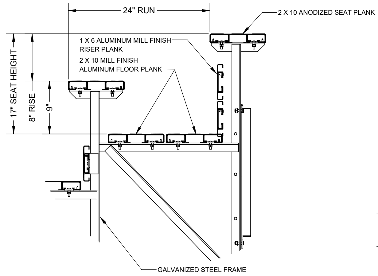
TYPICAL SEAT AND FOOT BOARD DETAIL NOT TO SCALE
