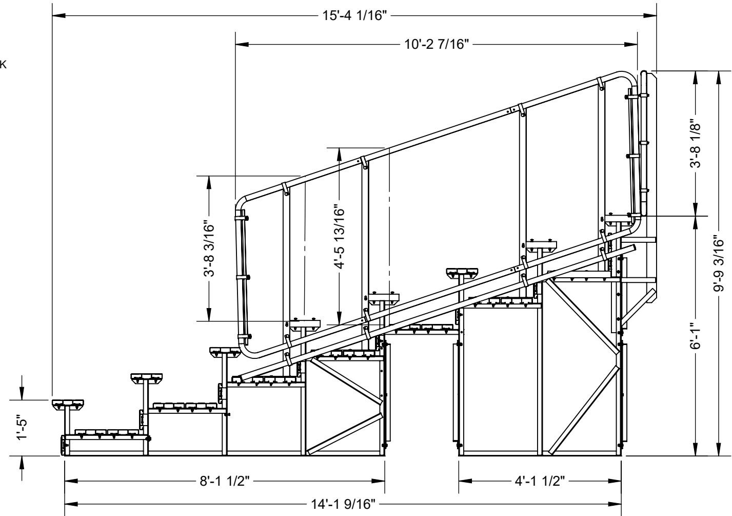
SECTION THROUGH BLEACHER SEATING
