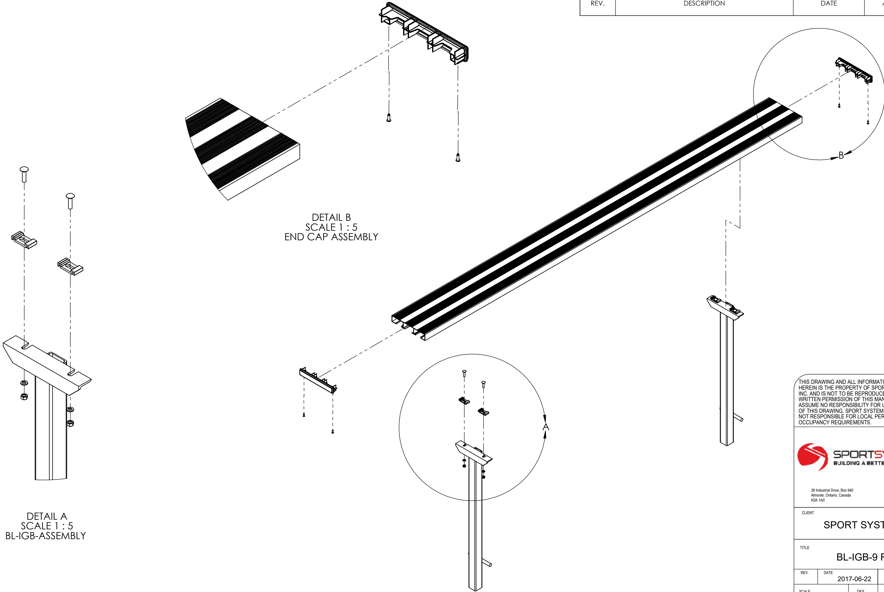
BL-IGB-9 FT. BENCH - EXPLODED VIEW - SHOWN
