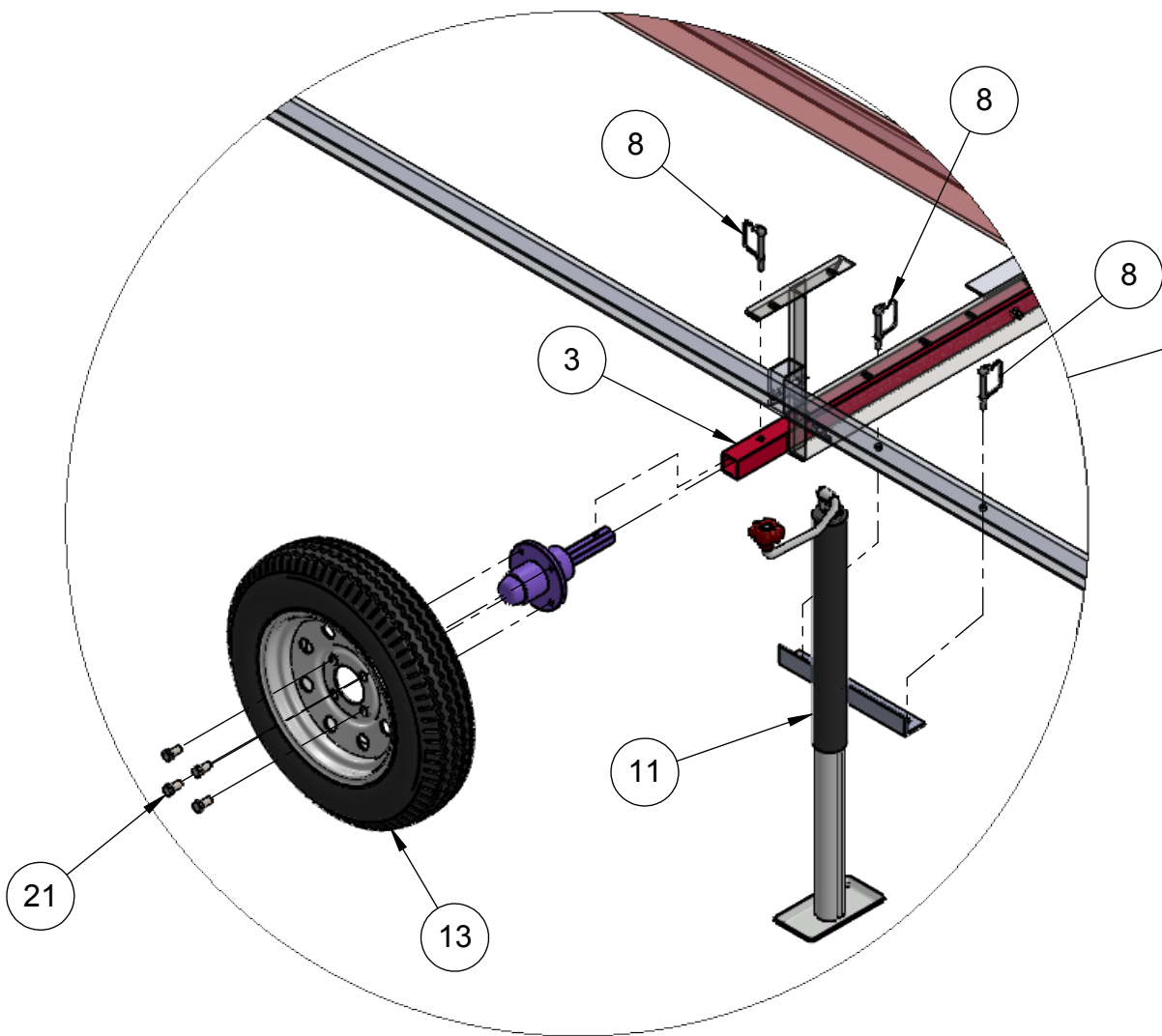
INSTALL DETAIL: AXLE HUB AND TIRE ASSEMBLY SCALE: 2:25
