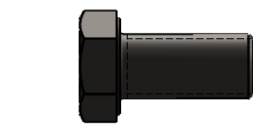
22 ISO 8676-M12 X 1.5 X 25-C
