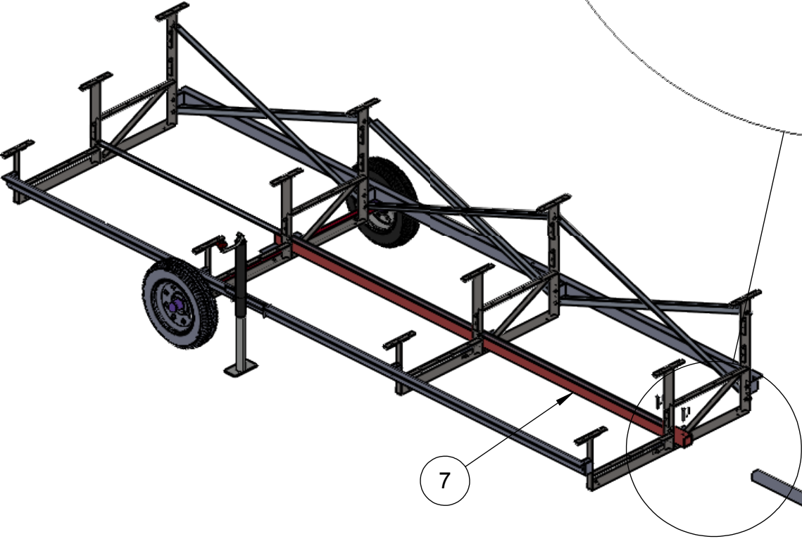
INSTALL DETAIL: TOW BAR SCALE: 1: 8
