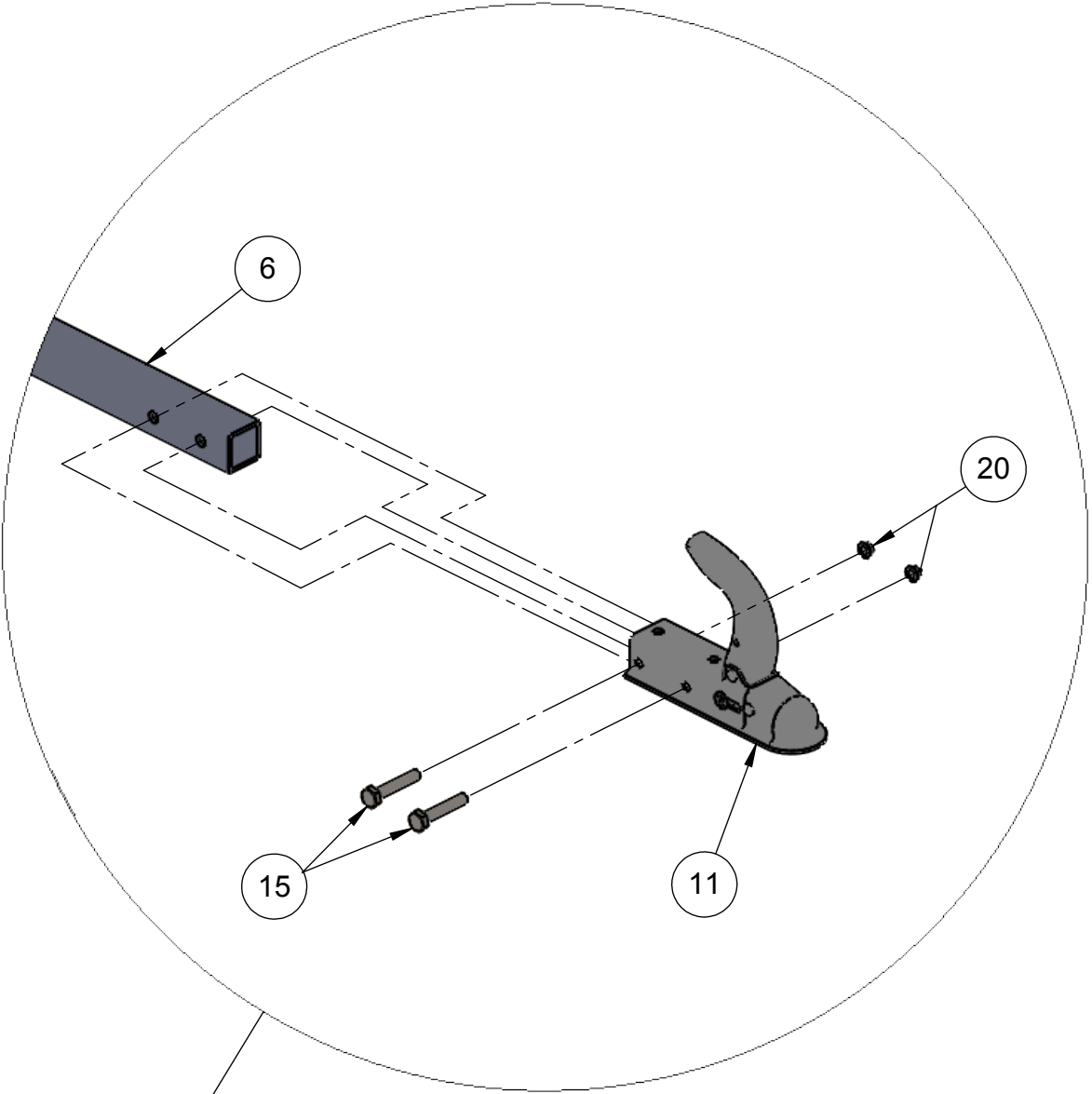
INSTALL DETAIL: 2" COUPLING SCALE: 1: 8
