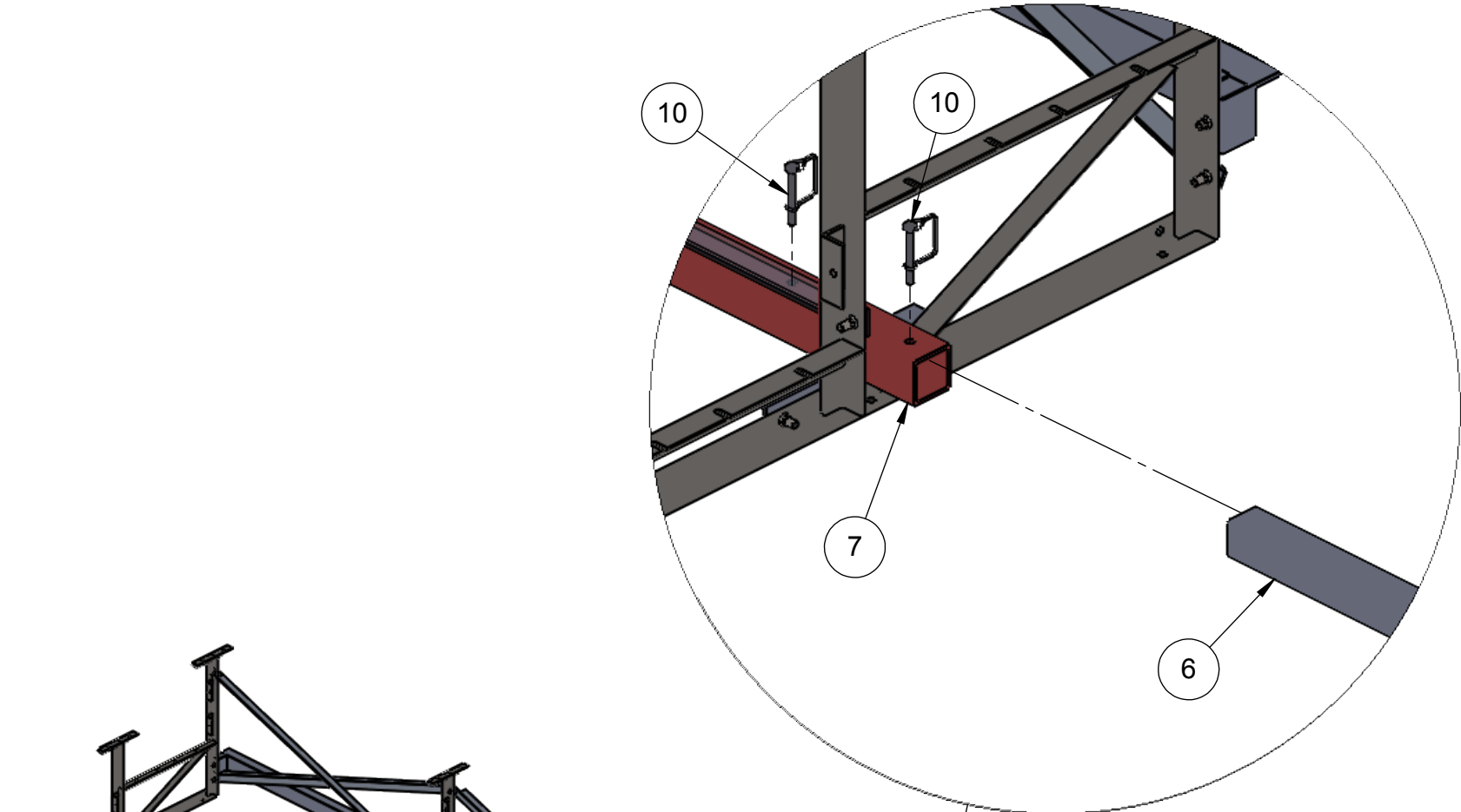
INSTALL DETAIL: TOW BAR SCALE: 1: 8
