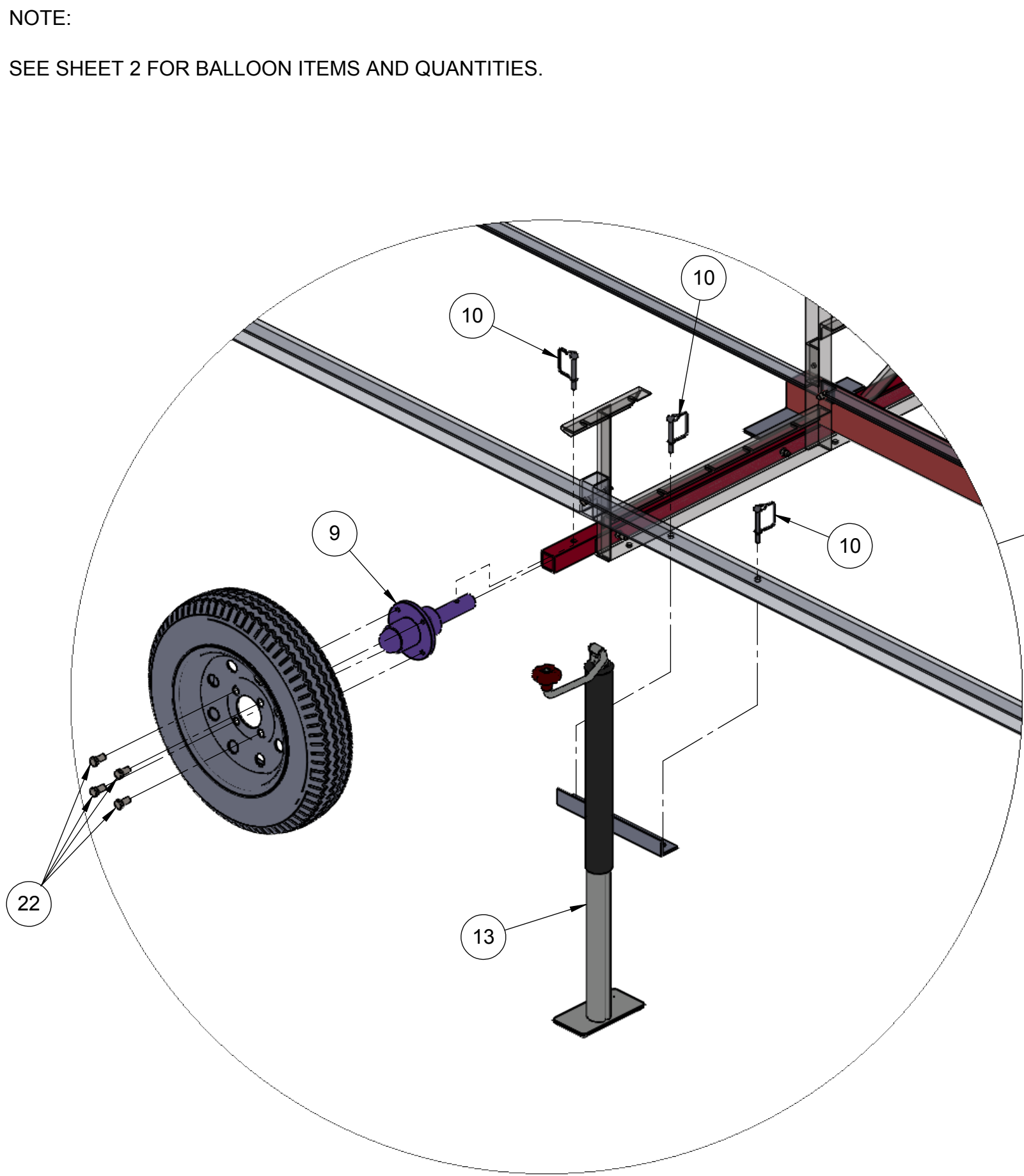
INSTALL DETAIL: AXLE HUB AND TIRE ASSEMBLY SCALE: 1: 10
