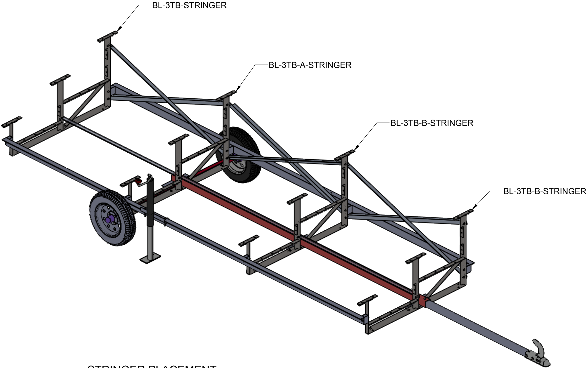
STRINGER PLACEMENT
