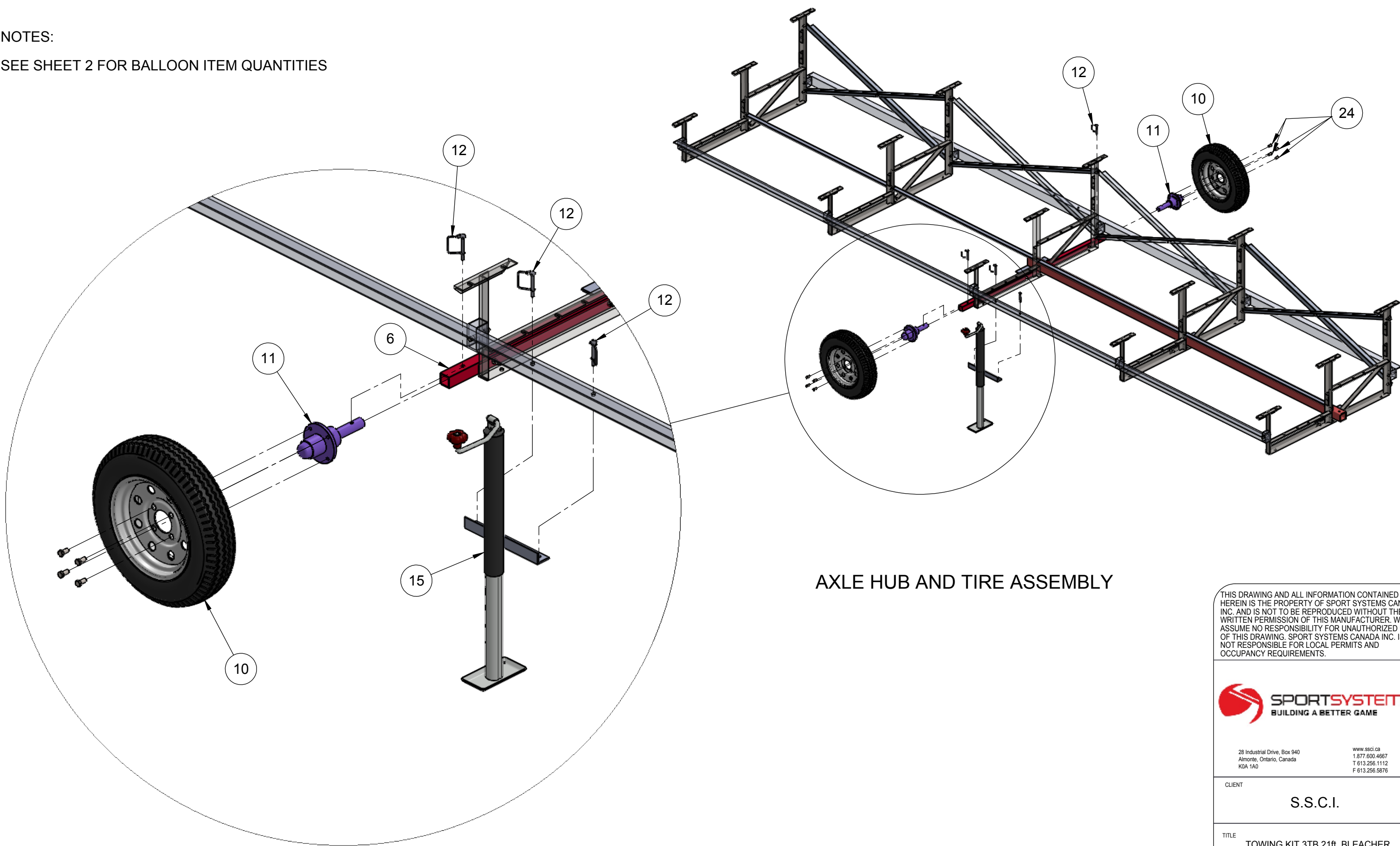
INSTALL DETAIL: AXLE HUB AND TIRE ASSEMBLY SCALE 1 : 10
