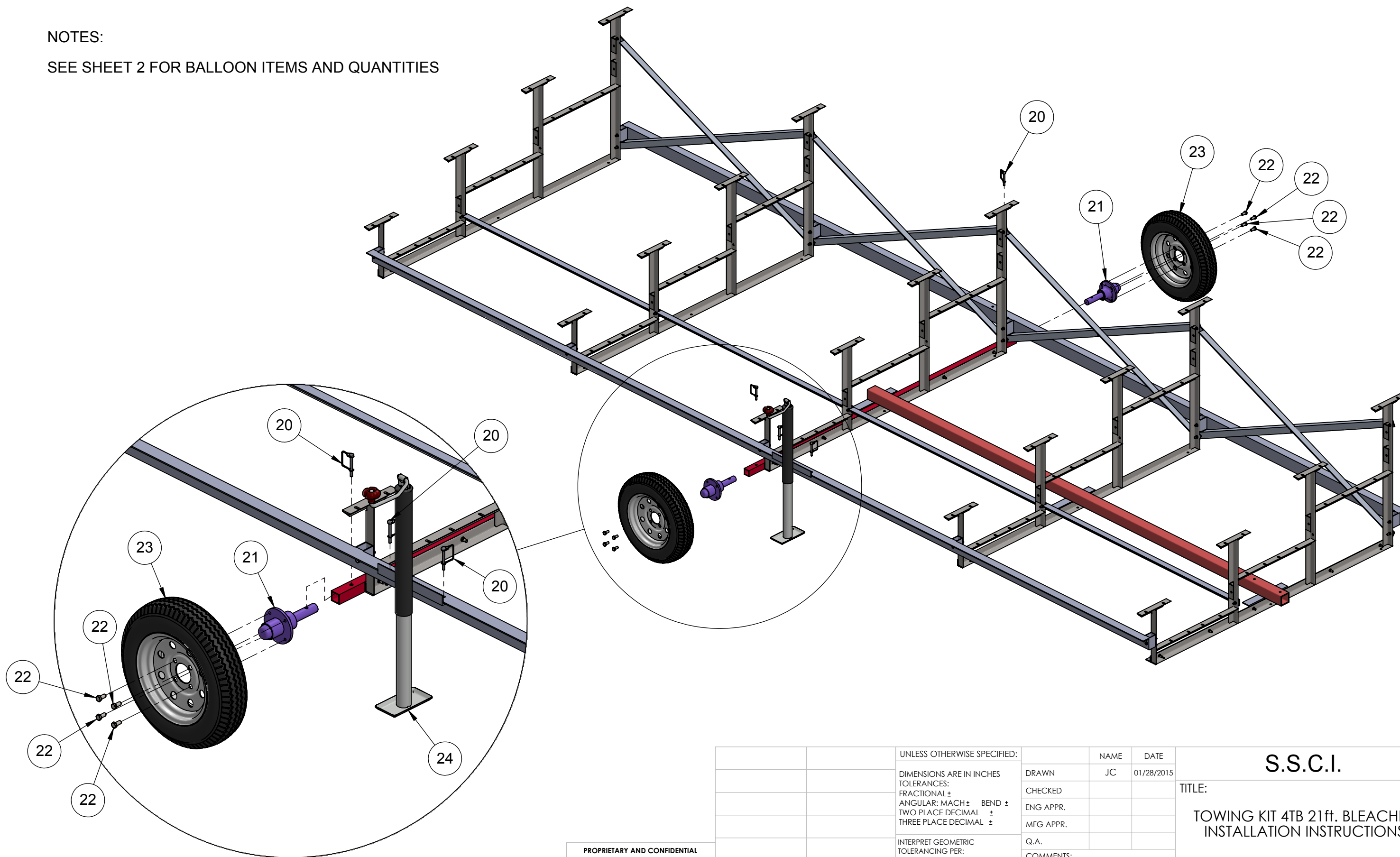
INSTALL DETAIL: AXLE HUB AND TIRE ASSEMBLY
