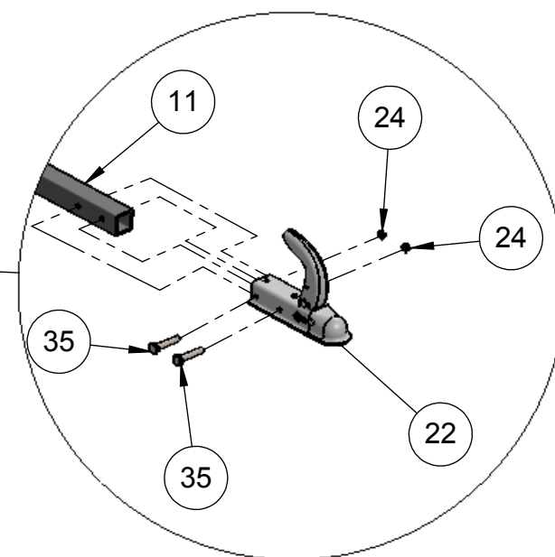
INSTALL DETAIL: 2" COUPLING SCALE 1 : 15
