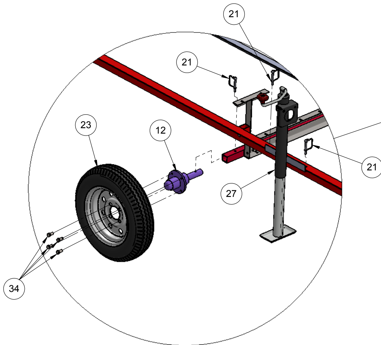
TYPICAL INSTALL DETAIL: AXLE HUB AND TIRE ASSEMBLY
