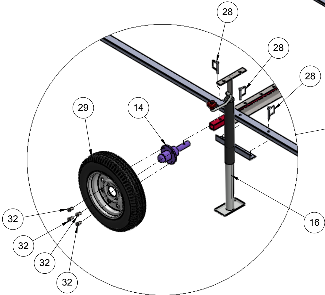
DETAIL: RIM AND TIRE ASSEMBLY
