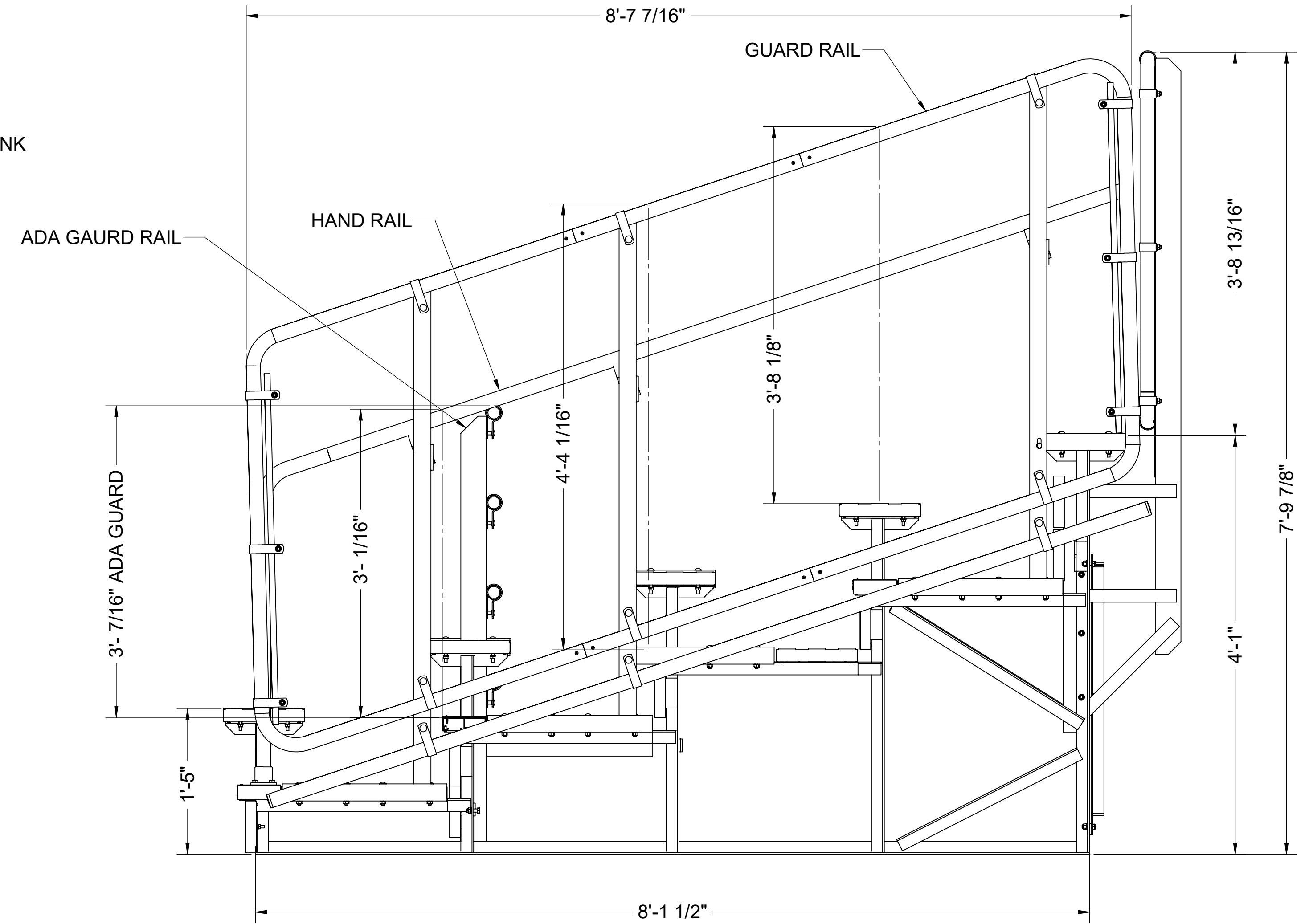
SECTION THROUGH BLEACHER SEATING NOTE: CHAIN LINK REMOVED FOR CLARITY
